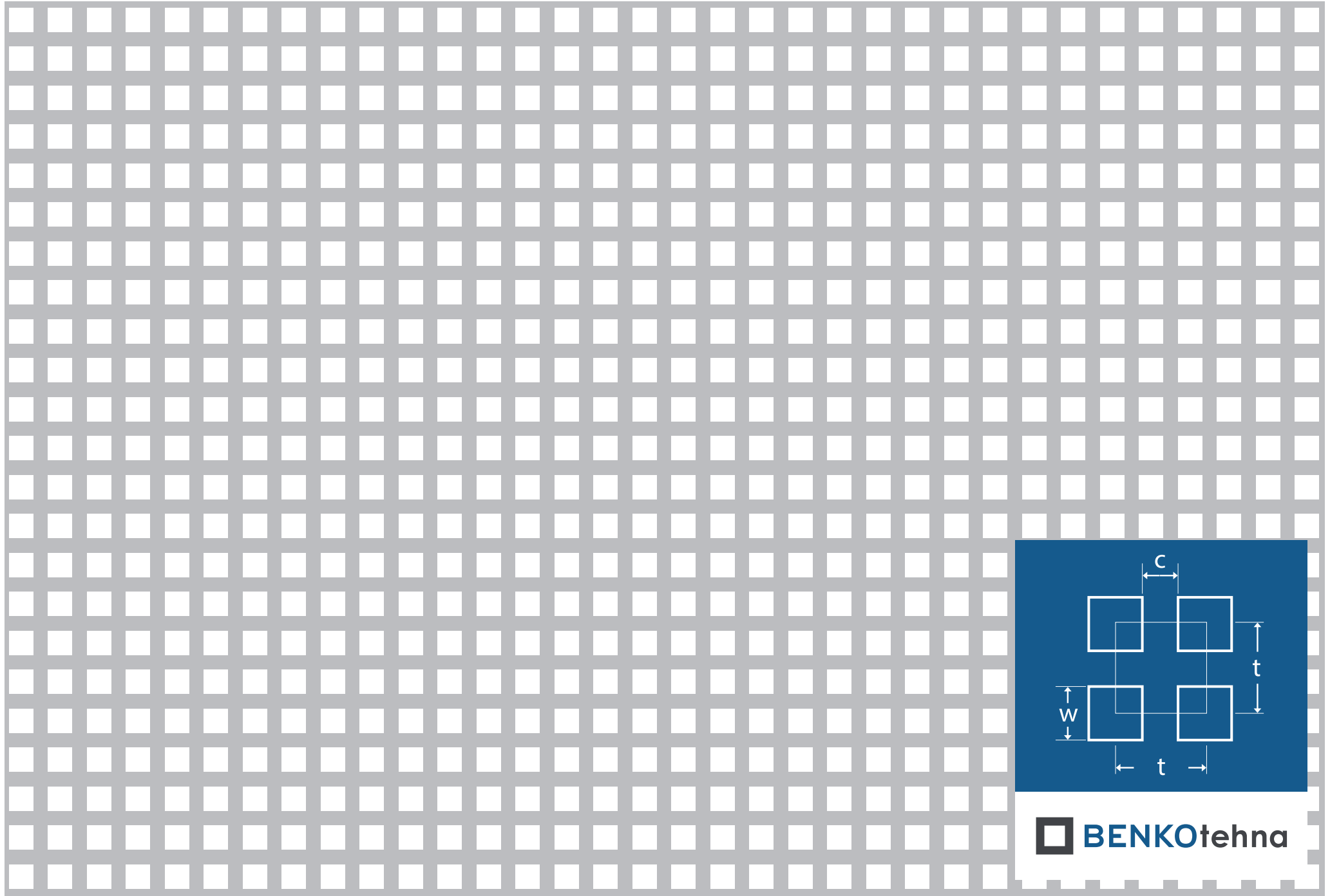
Kvadratna vrstna Kv 5-8: w = 5,0 \text{ mm} | c = 3,0 \text{ mm} | t = 8,0 \text{ mm} | odprtost = 39,06%
