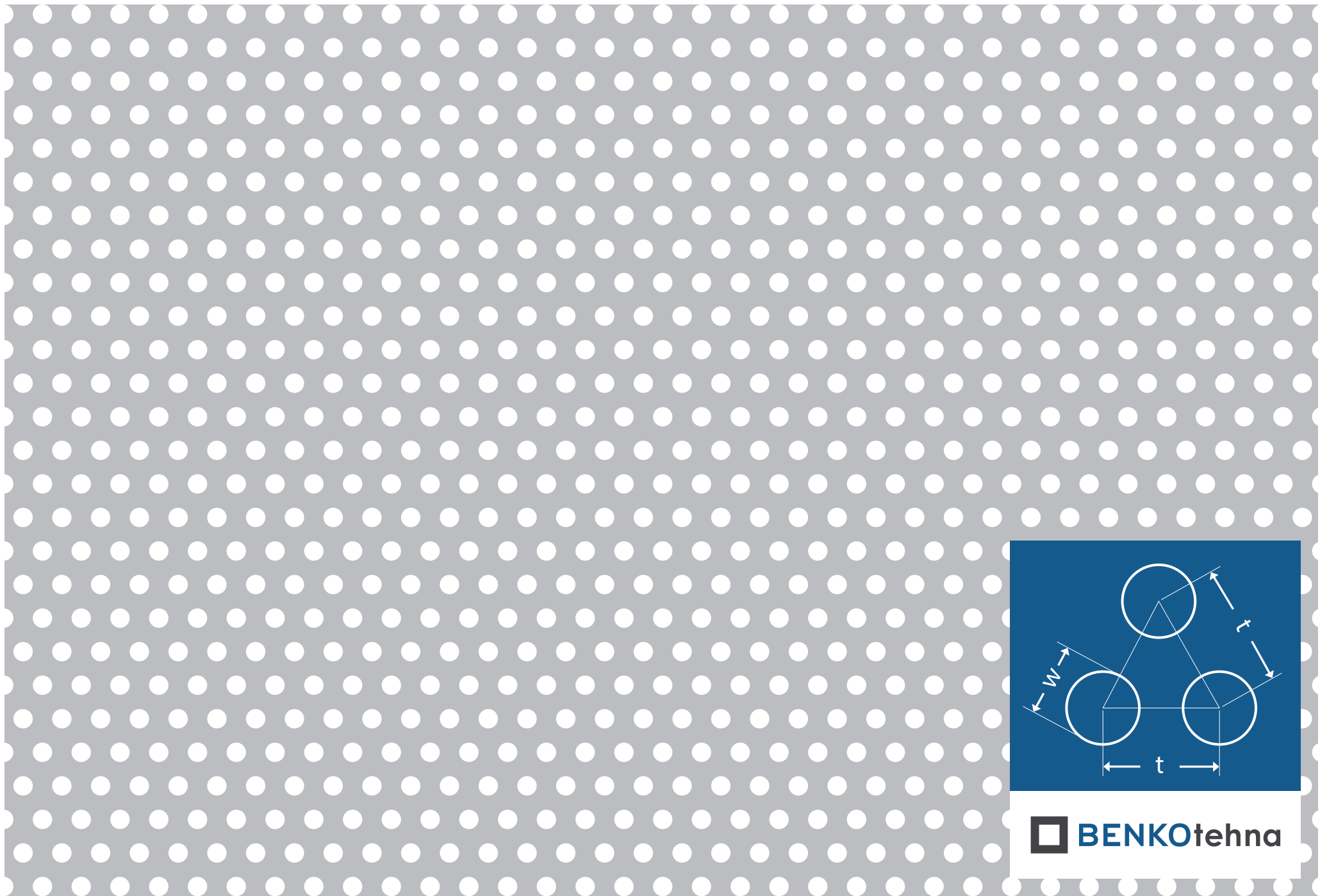
Okrogla zamaknjena Oz 4-8: w = 4,0 \text{ mm} | t = 8,0 \text{ mm} | odprtost = 22,68%
